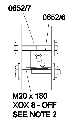
DETAIL 'B' SCALE 1:10
